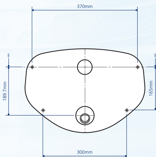
SINGLE SPOUT
