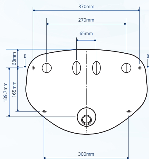
DUAL SPOUT
